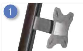
LCD Bracket - UB106-SMK1 LCD bracket is a specific design for use on Stealth - max. screen weight 5kg.
